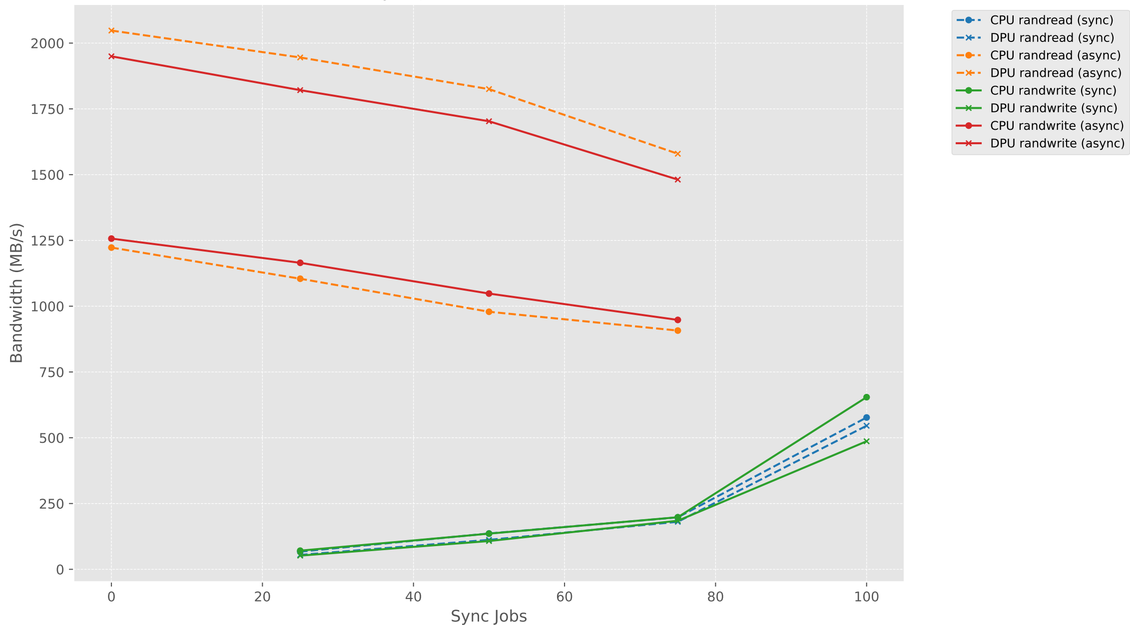
Bandwidth vs Sync Jobs (mixed) - RAND (CPU vs DPU)
